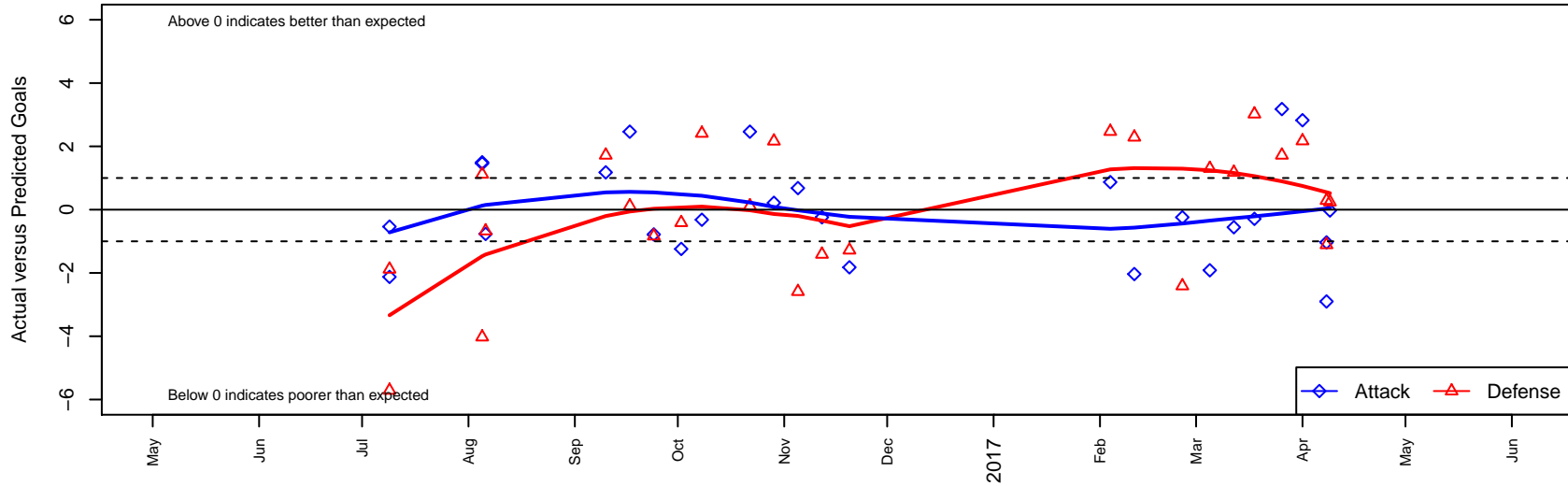
FC Bellevue B05 Dots are actual minus expected GF (blue circles) and GA (red triangles). Blue line is smoothed change in attack strength. Red is smoothed change in defense strength.
